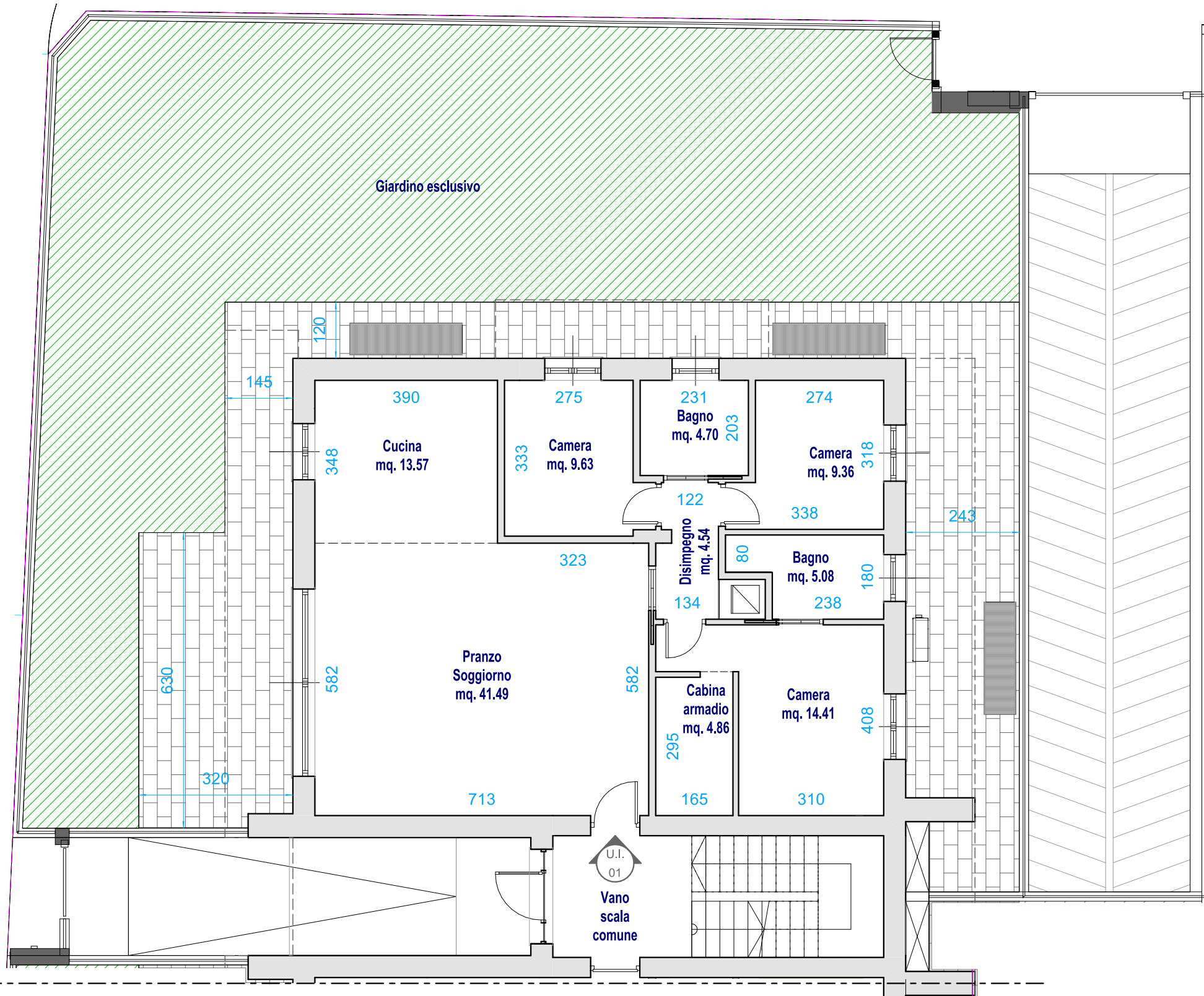
PIANO TERRA scala 1:100
